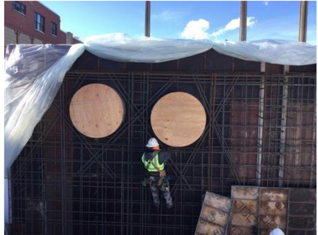
UG duct sleeves at gridline D foundation wall
