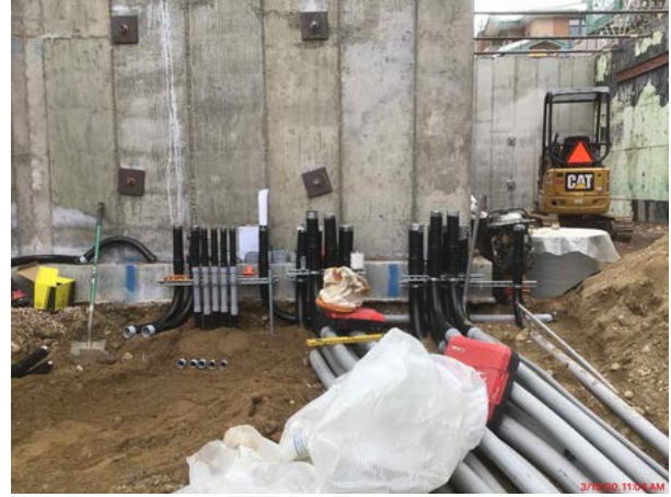
Underground MEP in progress
