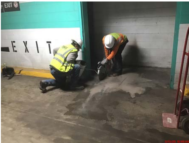
Garage slab being cut for new columns
